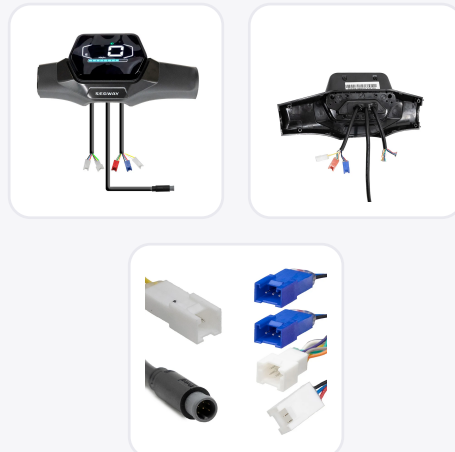
Display, rear view and connectors
