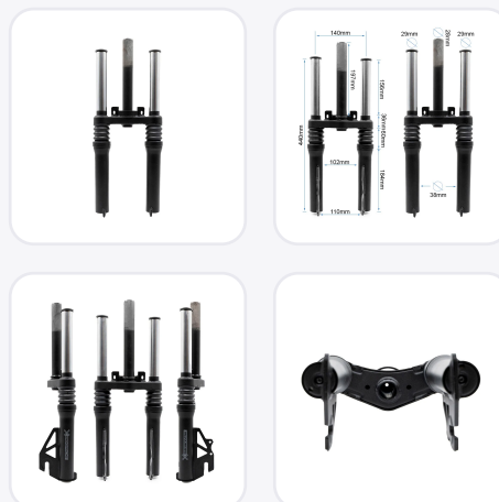
Damper views and dimensions
